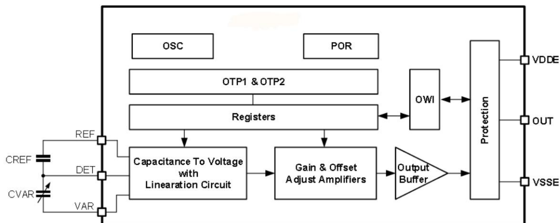
Fig. 2 Sensor Block Diagram
