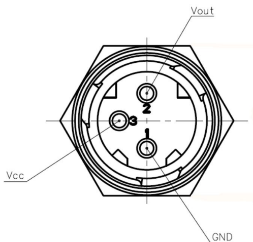
Fig. 1. PIN wire Schematic diagram
