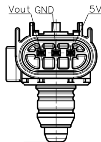
Fig.1 Pin diagram
